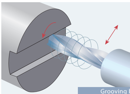
Grooving by Polar Coordinate Interpolation
