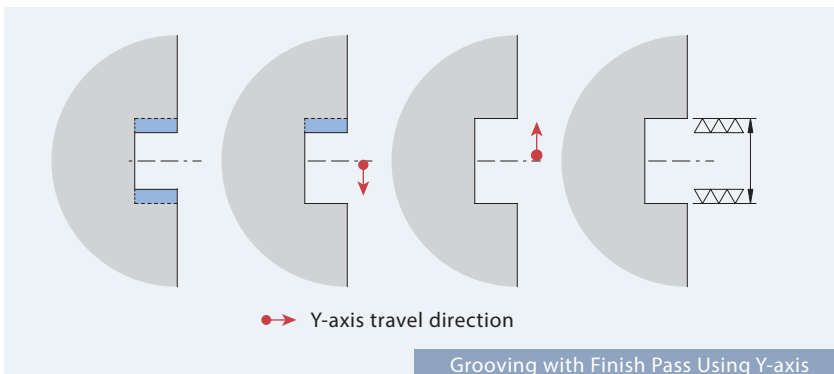
Grooving with Finish Pass Using Y-axis
